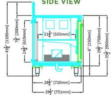
B - 28 1/4" D (720mm) SIDE VIEW
