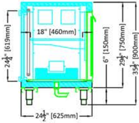
A - 24 1/2" D (625mm) SIDE VIEW
