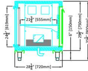
B - 28 1/4" D (720mm) SIDE VIEW
